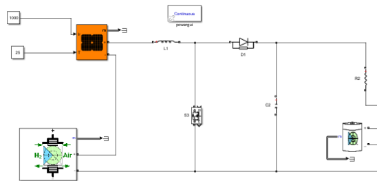
Figure 3: with one switch, one output
