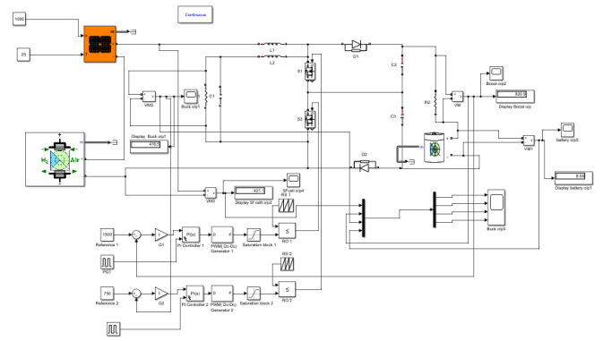
Figure 5: Simulation Diagram of Proposed Circuit of case 1
