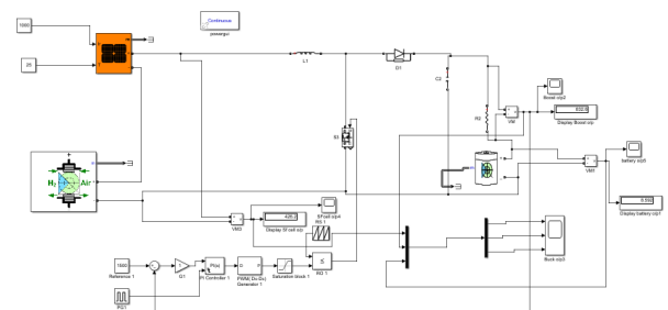
Figure 6: Simulation Diagram of Proposed Circuit of case 2
